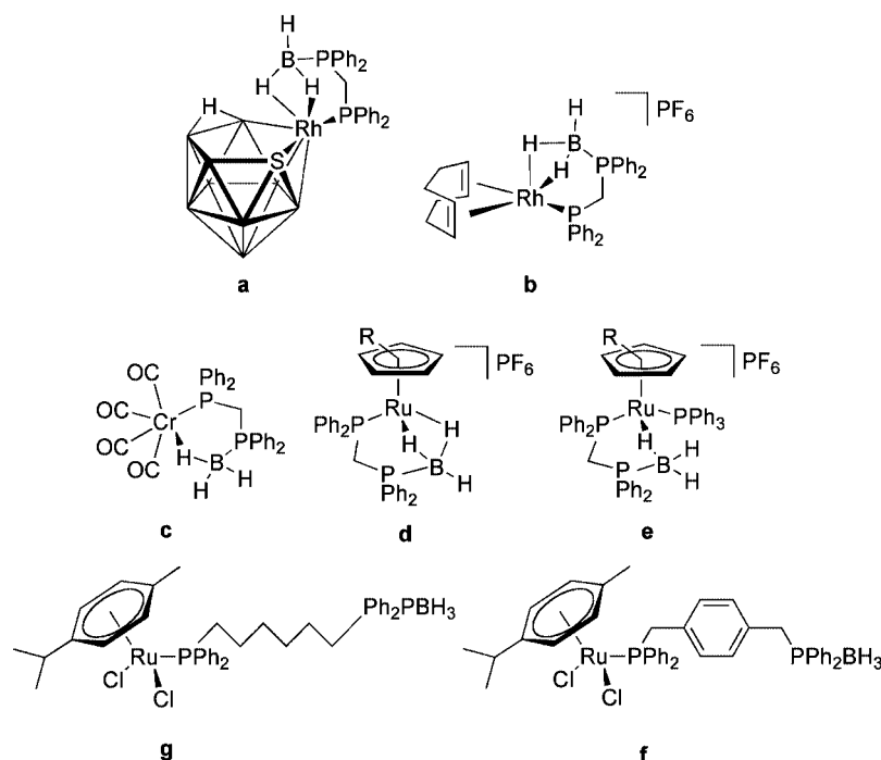
Figure 1. Examples of metal-containing phosphane–borane adducts.
