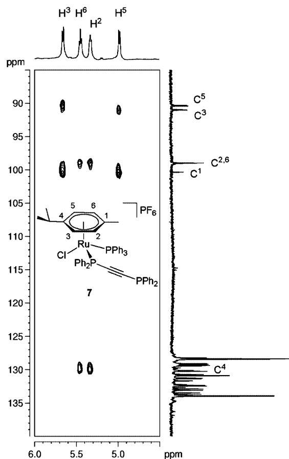
Figure 8. Section of the ^1\text{H} , ^{13}\text{C} long-range correlation NMR spectrum of 7 . Cross peaks originate from ^3J_{\text{CH}} couplings ( \text{CDCl}_3 , room temperature).
