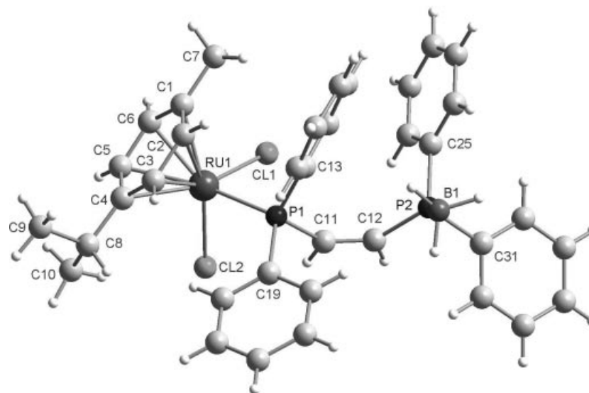
Figure 11. Ball-and-stick depiction of 2B in the solid state. Key bond lengths [Å] and angles [°]: Ru1–C11, 2.4107(8); Ru1–Cl2, 2.4307(8); Ru1–P1, 2.3424(8); C11–Ru1–Cl2, 88.11(3); C11–Ru1–P1, 83.32(3); Cl2–Ru1–P1, 86.28(3); Ru1–C avg , 2.22(4); Ru1–centroid, 1.7116(3); P1–C11, 1.823(3); P2–C12, 1.813(3); C11–C12, 1.327(4); P1–C11–C12, 139.3(3); P2–C12–C11, 135.3(3); P2–B1, 1.932(4).
