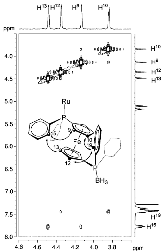
Figure 9. Section of the NOESY spectrum of 9B ( \text{CDCl}_3 , room temperature).
