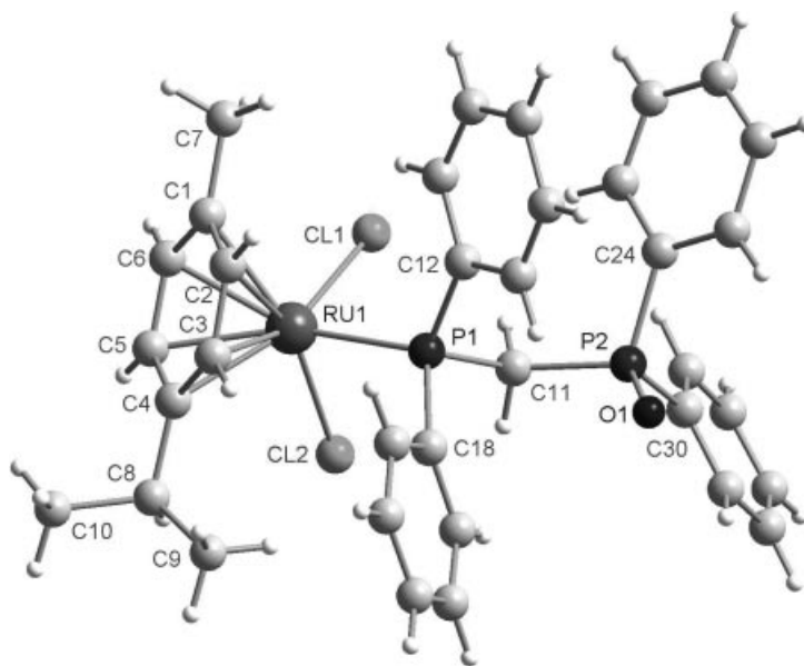
Figure 4. Ball-and-stick depiction of 3 in the solid state [selected molecule from the asymmetric cell]. Key bond lengths [Å] and angles [°] [averaged over asymmetric cell]: Ru–Cl, 2.432(7); Ru–Cl', 2.420(3); Ru–P, 2.355(7); Cl–Ru–Cl', 88.7(9); Cl–Ru–P, 87.2(9); Cl'–Ru–P, 83.4(8); Ru–C avg , 2.21(2); Ru–centroid, 1.700(5); P–C, 1.84(2); P'–C, 1.82(1); P–C–P', 120.6(7); P'–O, 1.49(1).
