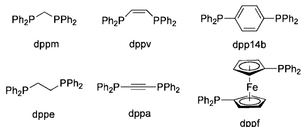
Figure 2. Bis(phosphane)s used in this study with their abbreviations.
