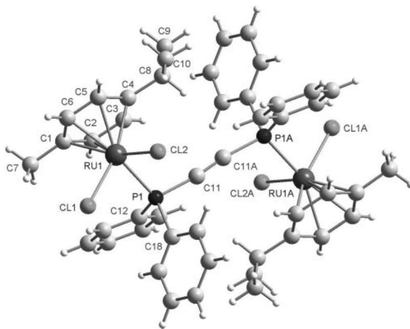
Figure 7. Ball-and-stick depiction of 6 in the solid state. Symmetry equivalent atoms, labeled with an A, are obtained by the symmetry operation -x, -y, 2 - z . Key bond lengths [Å] and angles [°]: Ru1–Cl1, 2.403(1); Ru1–Cl2, 2.204(1); Ru1–P1, 2.319(1); Cl1–Ru1–Cl2, 88.10(4); Cl1–Ru1–P1, 84.56(4); Cl2–Ru1–P1, 85.56(4); Ru1–C avg , 2.22(3); Ru1–centroid, 1.7045(3); P1–C11, 1.762(4); C11–C11#, 1.207(8); P1–C11–C11#, 172.4(5).
