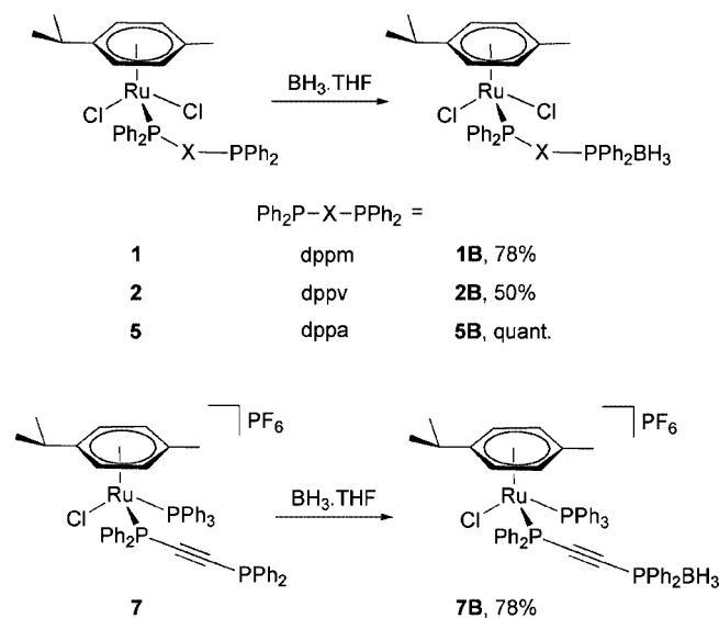
Scheme 2. Preparation of 1B , 2B , 5B and 7B .
