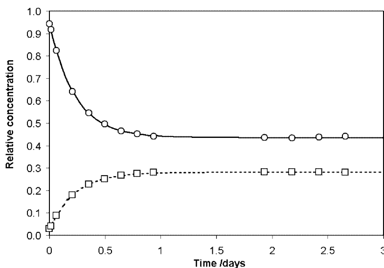
Figure 5. Equilibrium between complexes 5 and 6 at room temperature in \text{CDCl}_3 . Relative concentrations of 5 (circles) and 6 (squares) were determined by integration of ^1\text{H} NMR spectroscopic data. Note, the concentration of dppa is not shown as it is identical to that of 6 .
