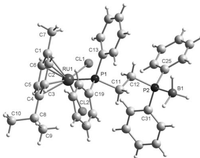
Figure 12. Ball-and-stick Depiction of 8B in the solid state. Key bond lengths [Å] and angles [°]: Ru1–C11, 2.436(2); Ru1–Cl2, 2.413(2); Ru1–P1, 2.356(2); C11–Ru1–Cl2, 88.86(5); C11–Ru1–P1, 90.42(6); Cl2–Ru1–P1, 84.49(6); Ru–C avg , 2.21(2); Ru1–centroid, 1.7005(5); P1–C11, 1.858(5); P2–C12, 1.817(6); C11–C12, 1.538(8); P1–C11–C12, 113.0(4); P2–C12–C11, 112.8(4); P2–B1, 1.933(8).
