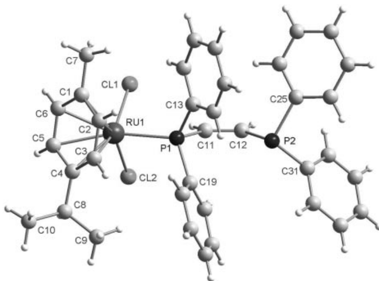
Figure 3. Ball-and-stick depiction of 2 in the solid state. Key bond lengths [Å] and angles [°]: Ru1–Cl1, 2.438(2); Ru1–Cl2, 2.418(1); Ru1–P1, 2.362(2); Cl1–Ru1–Cl2, 89.26(5); Cl1–Ru1–P1, 86.82(6); Cl2–Ru1–P1, 82.58(5); Ru1–C avg , 2.21(3); Ru1–centroid, 1.7002(4); P1–C11, 1.833(5); P2–C12, 1.845(5); C11–C12, 1.336(7); P1–C11–C12, 126.9(4); P2–C12–C11, 124.4(4).
