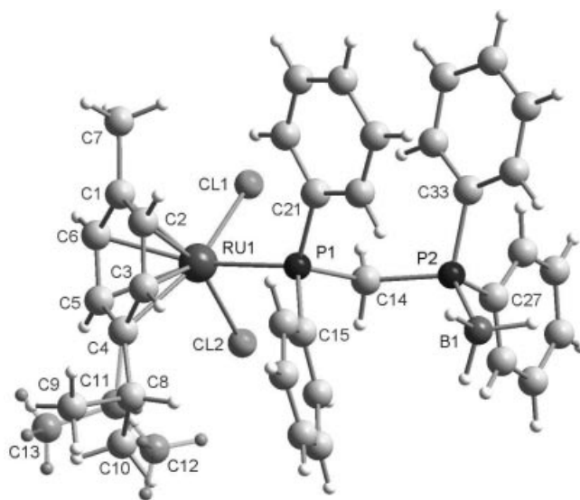
Figure 10. Ball-and-stick depiction of 1B in the solid state. The minor disordered component of the p -cymene ring is composed of atoms C11–C13. Key bond lengths [Å] and angles [ ^\circ ]: Ru1–Cl1, 2.417(2); Ru1–Cl2, 2.393(2); Ru1–P1, 2.351(2); Cl1–Ru1–Cl2, 85.65(8); Cl1–Ru1–P1, 86.47(9); Cl2–Ru1–P1, 87.33(8); Ru1–C avg , 2.19(3); Ru1–centroid, 1.7045(6); P1–C14, 1.831(8); P2–C14, 1.841(8); P1–C14–P2, 123.4(4); P2–B1, 1.91(1).
