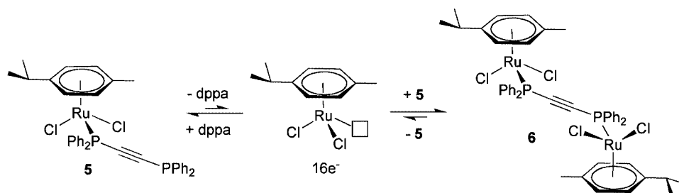
Scheme 1. Proposed mechanism for the equilibration of [(\eta^6\text{-}p\text{-cymene})\text{RuCl}_2(\eta^1\text{-dppa})] ( 5 ) with [(\eta^6\text{-}p\text{-cymene})\text{RuCl}_2(\mu\text{-dppa})\text{RuCl}_2(\eta^6\text{-}p\text{-cymene})] ( 6 ).
