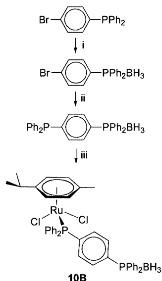
Scheme 4. Stepwise preparation of 10B . Reagents and conditions: i. \text{BH}_3 \cdot \text{THF} , 0^\circ\text{C} ; ii. \text{BuLi} , -78^\circ\text{C} , followed by \text{ClPPh}_2 ; iii. [(\eta^6\text{-}p\text{-cymene})\text{RuCl}_2]_2 , room temp.; overall yield: 50%.
