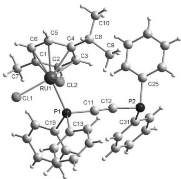
Figure 6. Ball-and-stick depiction of 5 in the solid state. Key bond lengths [Å] and angles [°]: Ru1–Cl1, 2.418(1); Ru1–Cl2, 2.402(1); Ru1–P1, 2.336(1); Cl1–Ru1–Cl2, 86.08(4); Cl1–Ru1–P1, 87.12(5); Cl2–Ru1–P1, 87.24(5); Ru1–C avg , 2.21(2); Ru1–centroid, 1.7006(5); P1–C11, 1.782(5); P2–C12, 1.765(6); C11–C12, 1.202(7); P1–C11–C12, 175.1(5); P2–C12–C11, 174.0(5).
